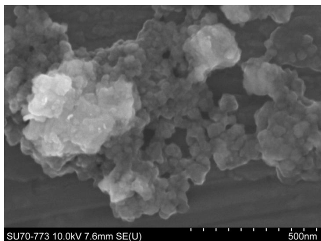
Figure 1. SEM image of ZnS prepared at 450 W.
