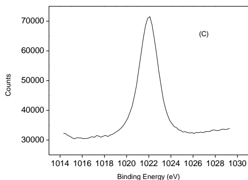
Figure 3. X-ray photoelectron spectra of the (a) S 2p (b) Zn2p 1/2 (c) Zn2p 3/2 peaks of ZnS450W.
