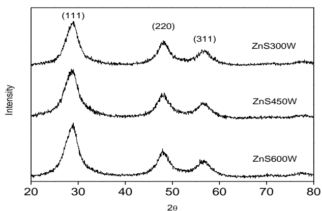
Figure 2. X-ray diffraction spectra of ZnS samples prepared via microwave irradiation.
