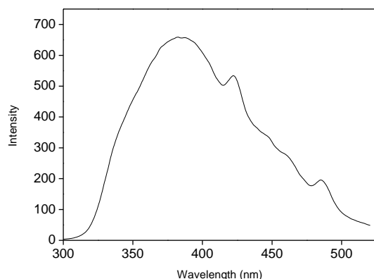
Figure 5. Luminescence spectra of ZnS450W excited at 275 nm.
