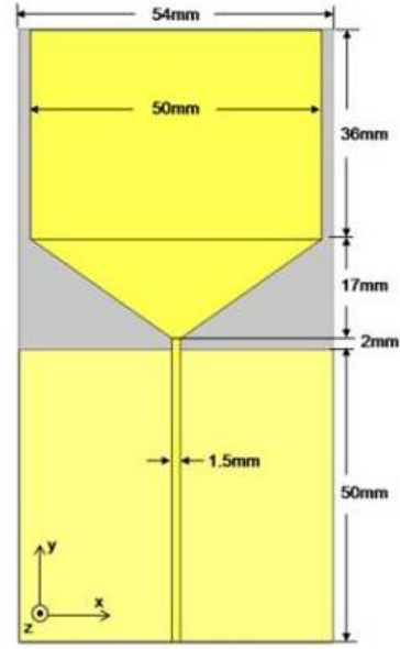
Figure 2: Antenna geometry.
