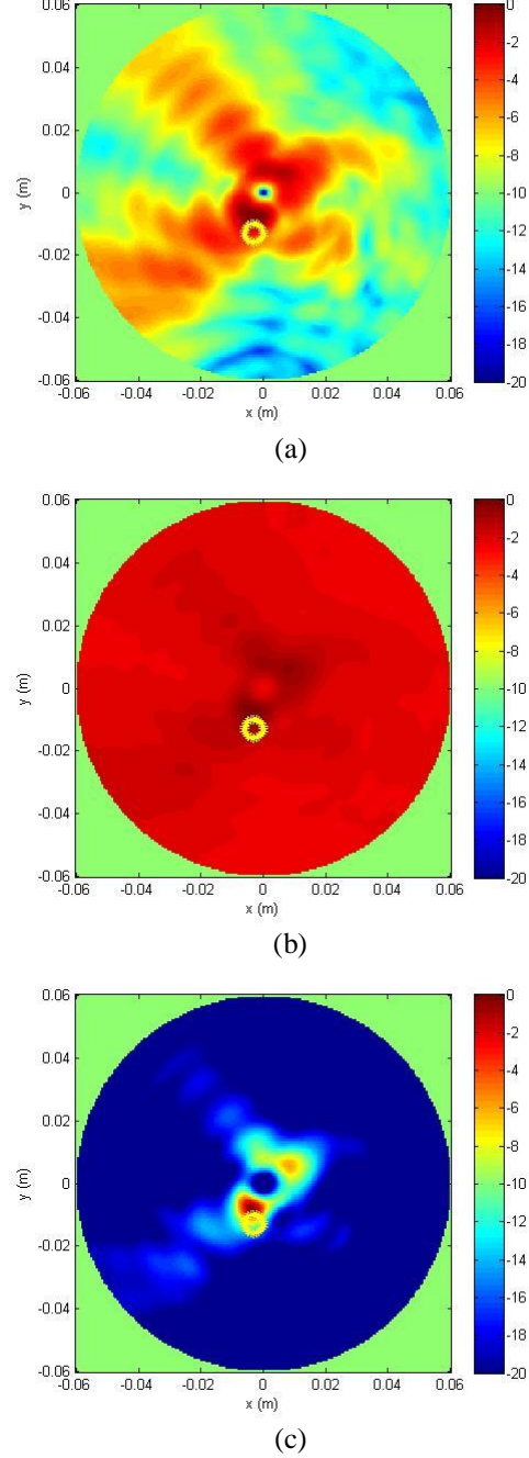
Figure 3: Reconstructions in the presence of 5-mm tumor (marked with yellow circle) by: a) Non-coherent Migration b) WB MUSIC c) Interferometric MUSIC.
