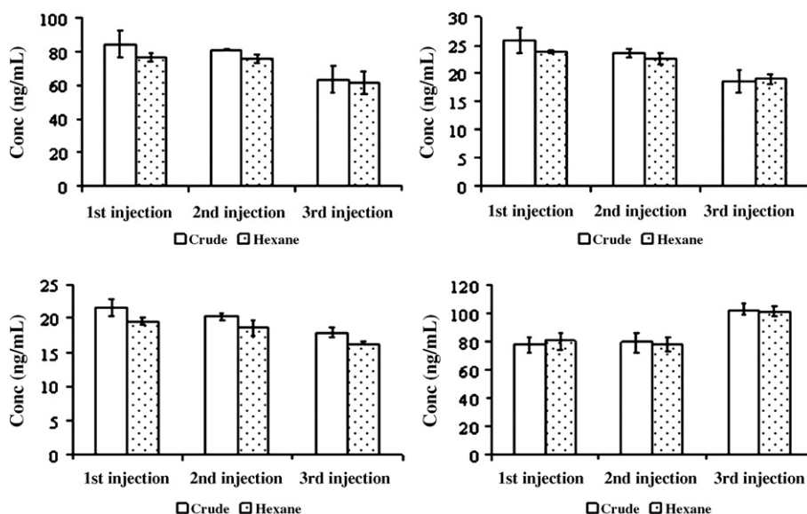
Fig. 2. Average concentrations of AZAs ( n = 3 ) obtained by injection of three successive LRM extracts and three successive LRM extracts after hexane partitioning on the TSQ. Each series of three injections were separated by the injection of three successive standard solutions. (A) Concentration of AZA1 in partitioned and non-partitioned LRM. (B) Concentration of AZA2 in partitioned and non-partitioned LRM. (C) Concentration of AZA3 in partitioned and non-partitioned LRM. (D) Concentrations of AZA1 standards (104 ng/mL) after the injection of three LRM and three partitioned LRM.
