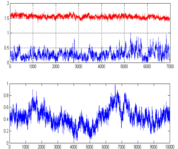
Figure 6: Above: Plot of the wind velocity given in Figure 4 after normalization (blue) and the Lévy index (red) obtained using a moving window is size 1024 elements. Below: Simulated wind velocities computed for Lévy index \gamma = 1.55
