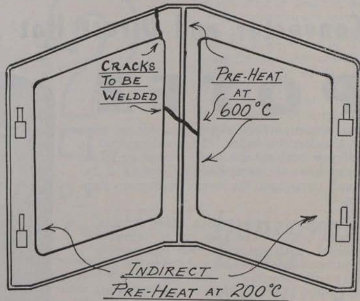
FIG. 2 FRACTURED BOILER DOOR FRAME
