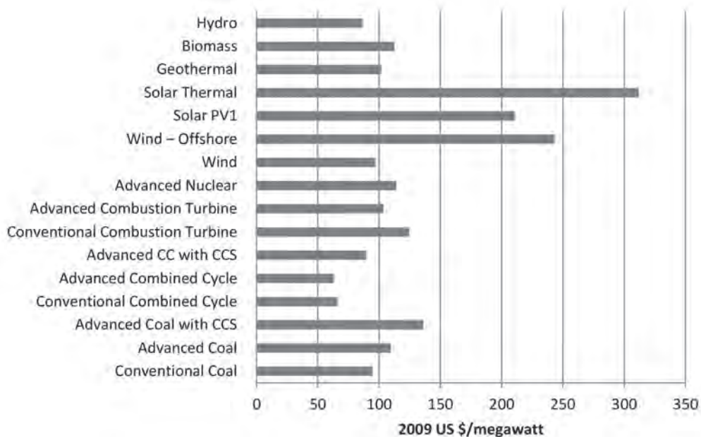
Figure 7.5. Total System Levelized Cost of New Generation Resources, 2016. 5
