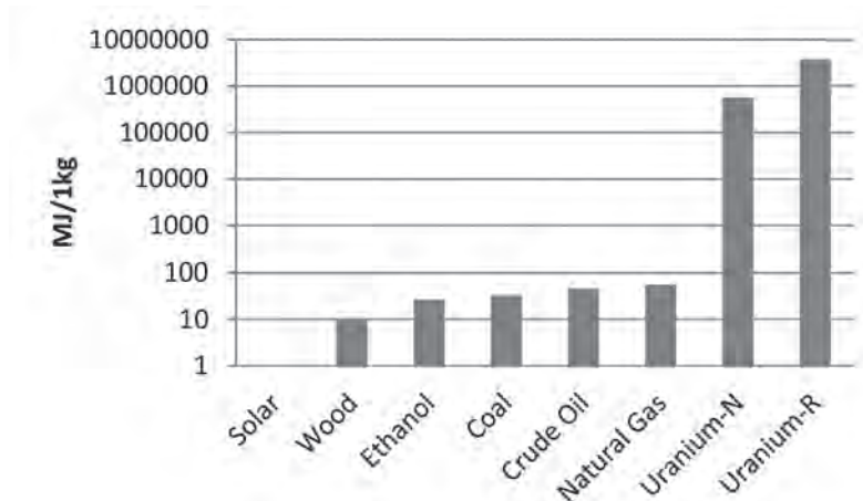
Figure 7.3. Energy Densities of Major Fuel Sources. 4 Uranium-N and Uranium-R Stand for Natural Uranium and Reactor-graded Uranium, Respectively.
