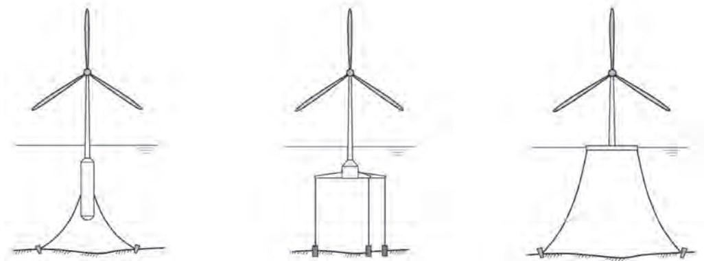
Figure 4.4. Single FOWT Systems: (a) S-FOWT, (b) TLP-FOWT, and (c) B-FOWT. 13
