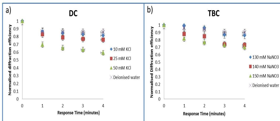
Figure 4. Normalised diffraction efficiency change response DC and TBC plasticised PVC photonic structures (a) KCl exposure to (10-50 mM) (b) NaNO 3 exposure to physiological levels (130mM-150mM)
