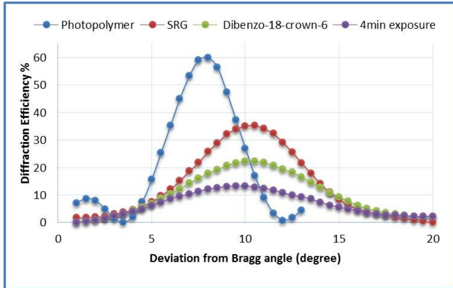
Figure 2. Bragg curves with spatial frequency centred at 300 l/mm recorded in layers with thickness of 30 \mu\text{m} on a glass slide taken for the photopolymer before and after thermal treatment, after spin coating with dibenzo-18-crown-6 (DC) functionalising material and after exposure to analyte \text{K}^+
