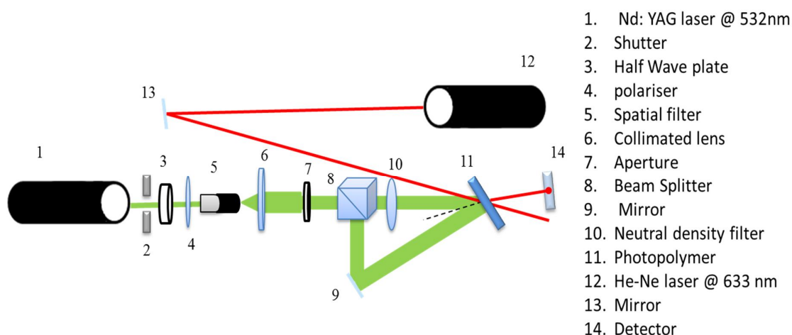
Figure 1. Experimental set-up for recording transmission holograms
