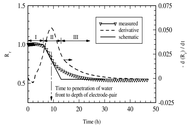
Figure 3: Schematic for R_r during absorption and derivative to estimate time of arrival of water-front.
