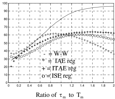
Fig. 5. Phase margin
