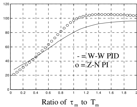
Fig. 8. Phase margin comparison
