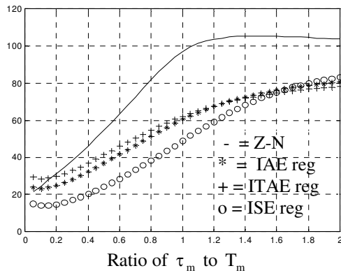
Fig. 2. Phase margin
