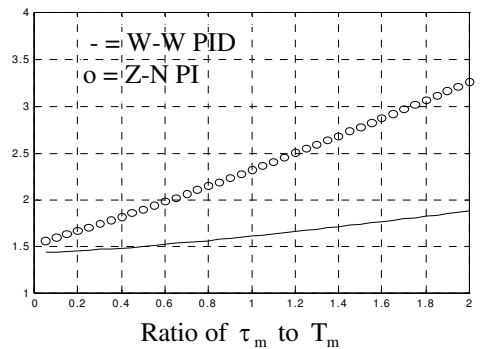
Fig. 7. Gain margin comparison
