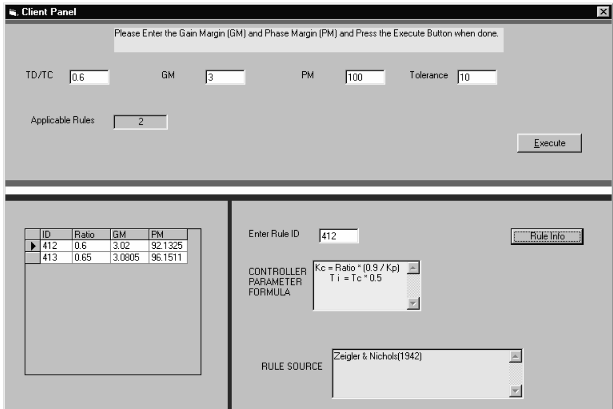
Fig. 9: Main User Screen
