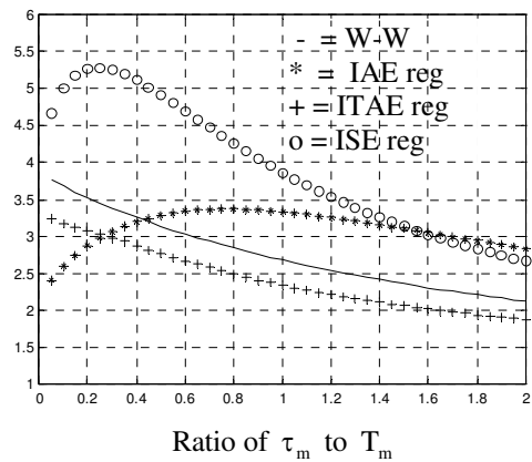
Fig. 6. Maximum sensitivity
