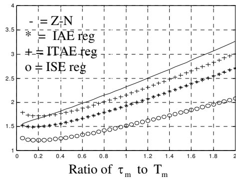
Fig. 1. Gain margin
