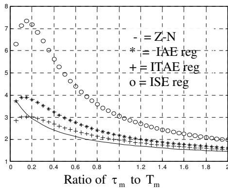
Fig. 3. Maximum sensitivity
