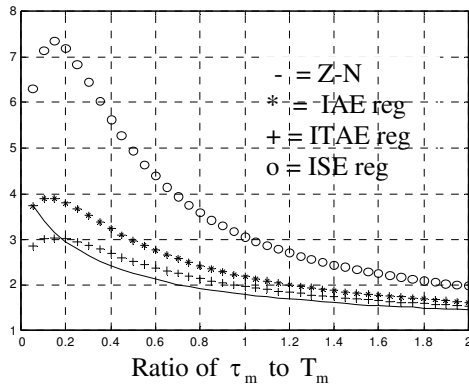
Fig. 3. Maximum sensitivity
