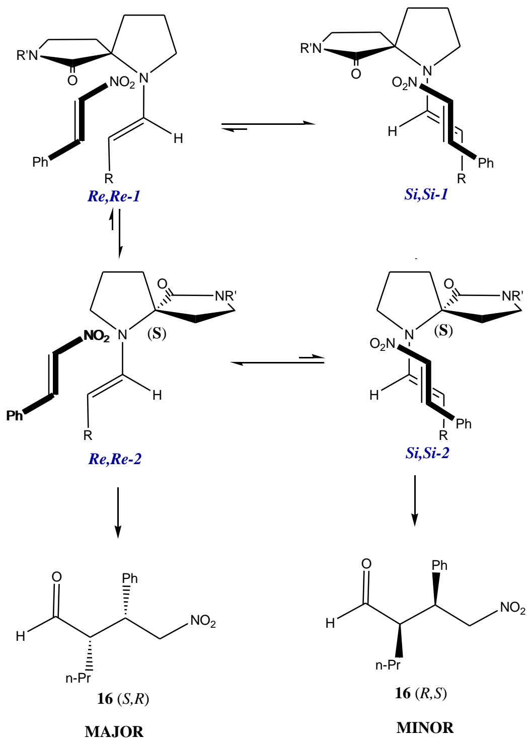
Figure 4. Proposed transition state model for Michael addition reaction of valeraldehyde with \beta -nitrostyrene using spirocyclic lactam catalysts.
