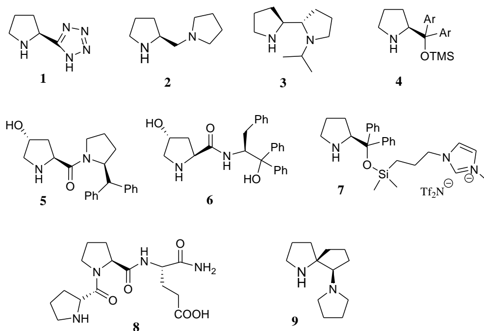
Figure 1. Proline and 4-hydroxyproline derived organocatalysts. 1-6
