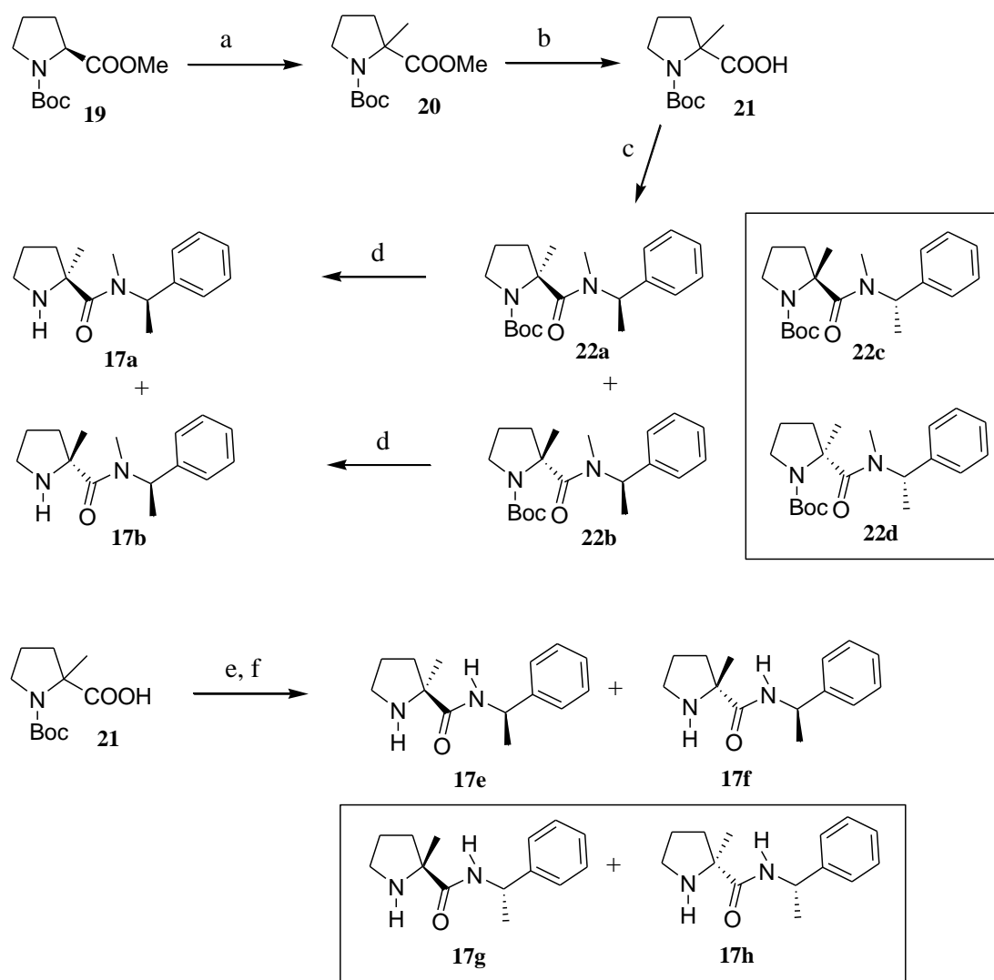
Scheme 1: Reagents and conditions; (a) i) LiHMDS, THF, -78\text{ }^{\circ}\text{C} , ii) methyl iodide, rt, 72%; (b) i) NaOH, MeOH/H 2 O, reflux, ii) 1M HCl, 93%; (c) (R) - N , \alpha -dimethylbenzylamine, DIPEA, HATU, DMF, rt, 49%; (d) 50% TFA in DCM, rt, 88-92%; (e) (R) - \alpha -methylbenzylamine, DIPEA, HATU, DMF, rt, 94%; (f) 50% TFA in DCM, rt, 93-96%.
