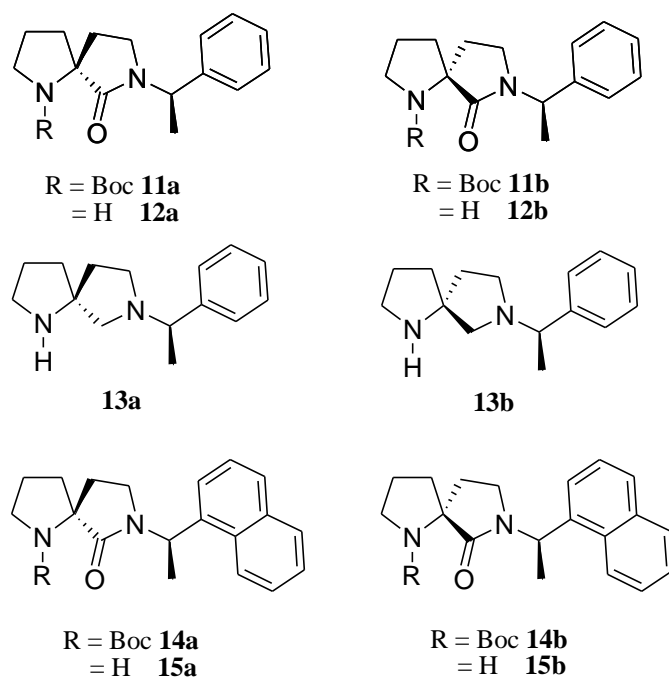
Figure 2. Synthesised spiro lactam and spiro diamine organocatalysts
