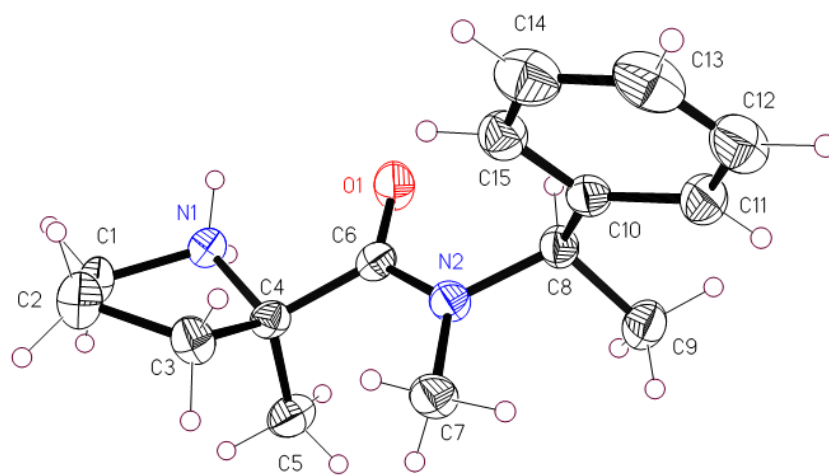
17b ( R,R )
