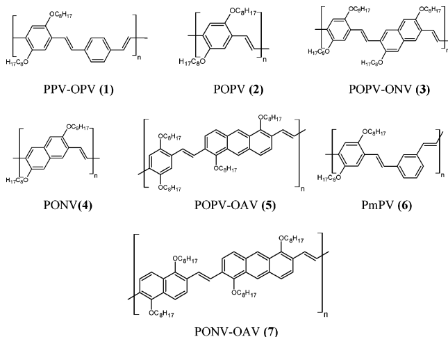
Figure 1. Polymer structures 1–7.
