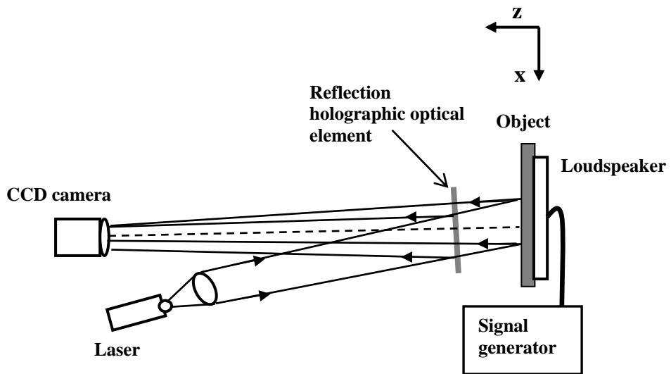
Fig.3. ESPI system with a holographic optical element only 7
