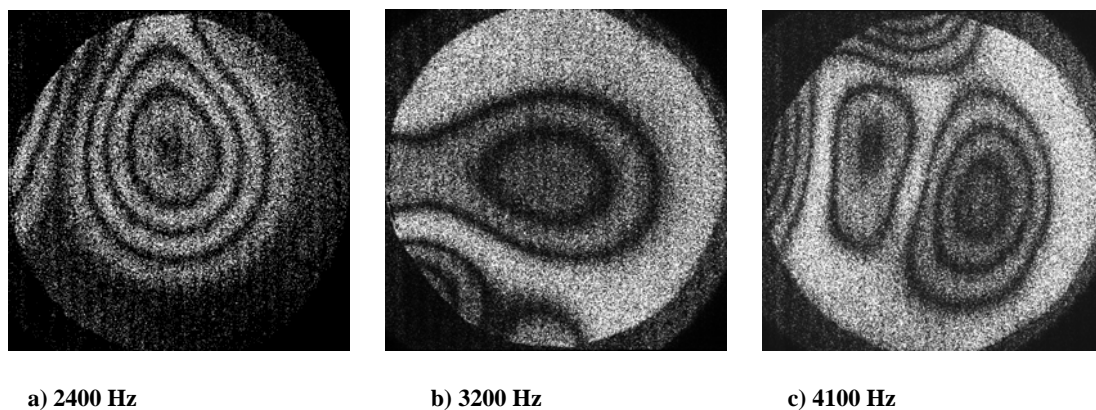
Fig.5. ESPI vibration modes of an aluminium diaphragm recorded with the ESPI system with one HOE only. The amplitude of the sinusoidal signal driving the loudspeaker is 1 V. The field of view is 40 mm x 40 mm.
