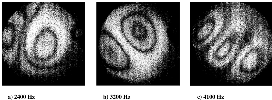
Fig.4. ESPI vibration modes of an aluminium diaphragm recorded with the ESPI system with HOE and partially reflective glass plate. The amplitude of the sinusoidal signal driving the loudspeaker is 1 V. The field of view is 40 mm x 40 mm.
