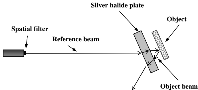
Fig. 1. Recording of the reflection hologram using the Denisyuk method.
