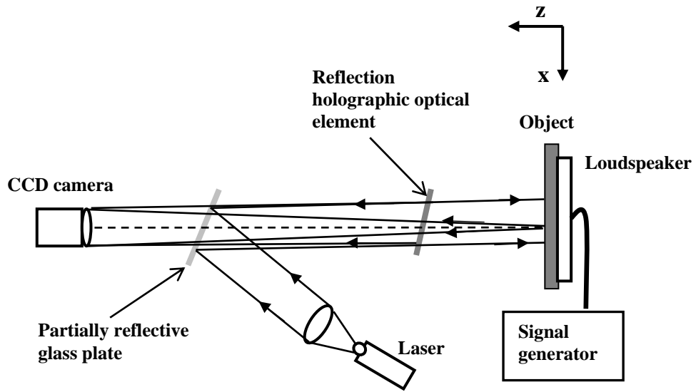
Fig.2. ESPI system with a holographic optical element and a partially reflective glass plate 6
