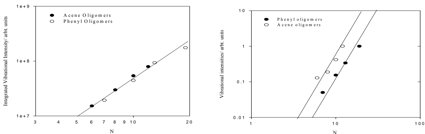
Figure 3a/3b. Integrated Raman intensity plotted against N . Figure (a) integrated from 100 - 3200\text{cm}^{-1} ; figure (b) the relative intensities of the C=C vibrational modes along the backbone. The solid lines show slopes of 2(a) and 4(b).
