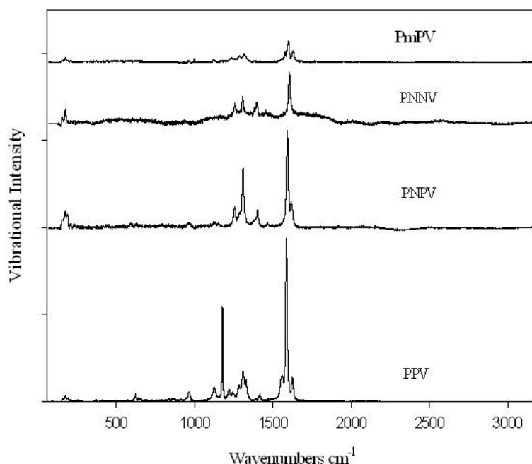
Figure 6. Polymer Raman spectra (offset for clarity)
