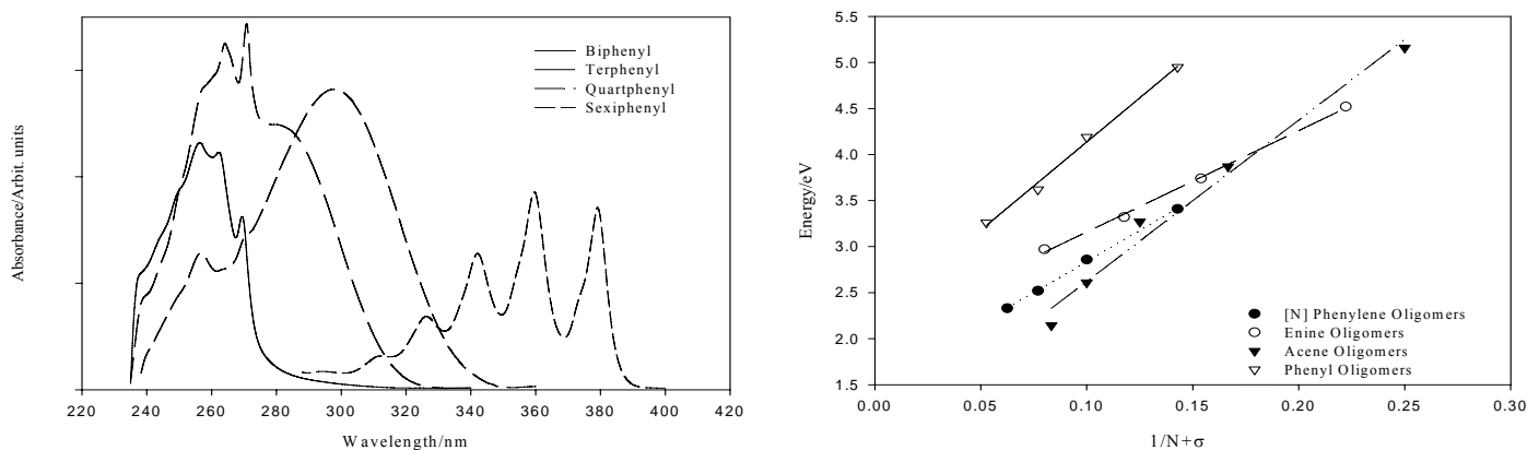
Figure 2a/2b. Position of maximum absorbance against 1/(N+\sigma) and Progression of Phenyl oligomers from 2 to 6 repeat units.
