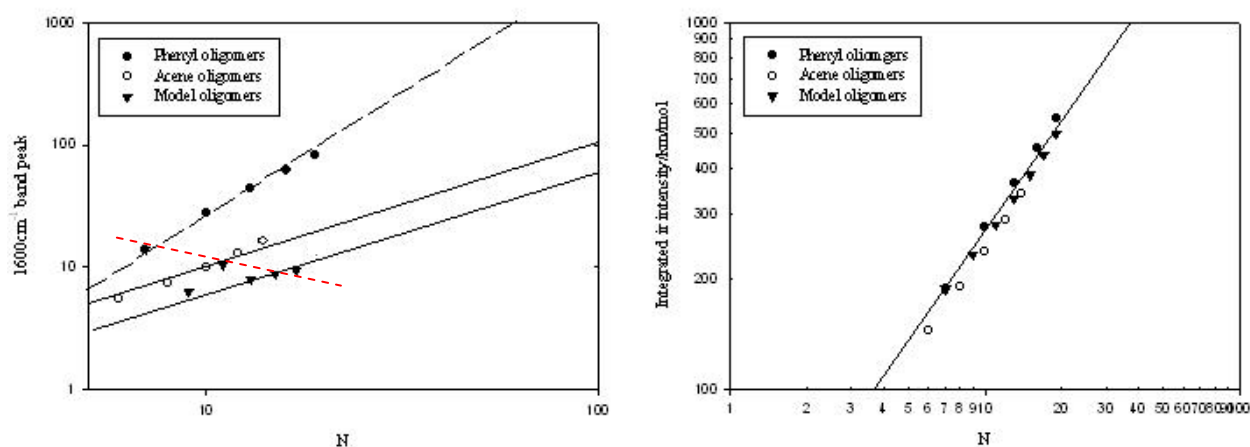
Figure 5a/5b. Integrated IR intensity plotted against N. Figure (a) the relative intensities of the C=C vibrational modes along the backbone; figure (b) integrated from 100-3500cm -1 . The solid lines show slopes of 1 and the dotted line shows a slope of 2.
