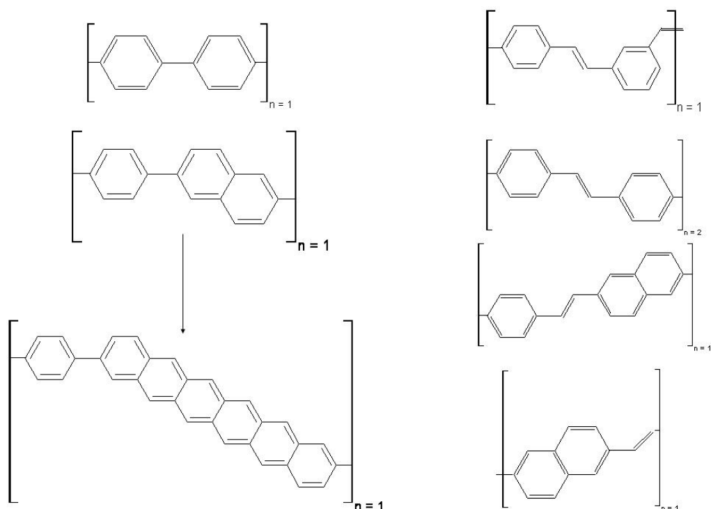
Figure 4 Structures of model oligomers (1MO→5MO), left, and synthesised polymers, right. The [ ] n=1 is not really right.
