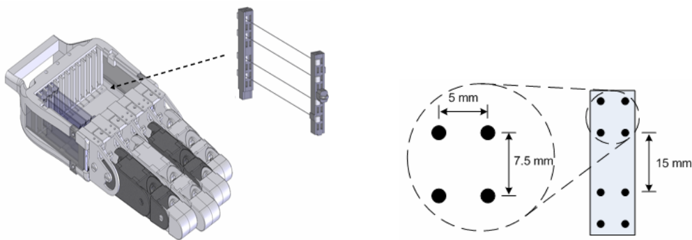
Figure 1: SMA Actuated Hand Prototype & SMA Bundle Figure 2: SMA Bundle Dimensions
