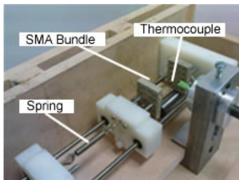
Figure 3: SMA Layout in Test Rig ( h -value setup)
