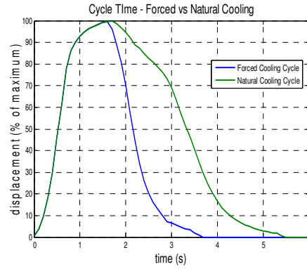
Figure 10: Forced (Al) & Natural Cooling
