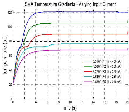
Figure 5: SMA Temperature Gradients
