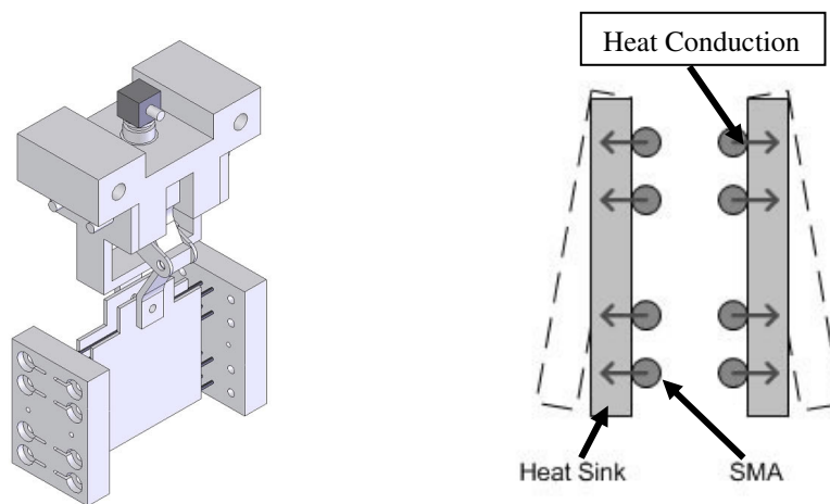
Figure 7 – Cooling Module Attachment (Closed) Figure 8 – Heat Conduction using Heat Sink
