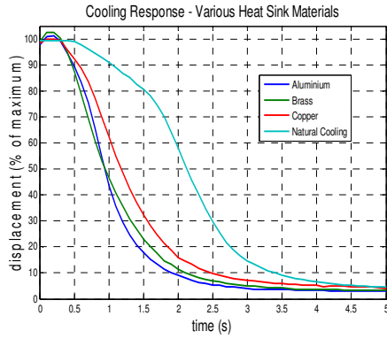
Figure 9: Cooling Response due to Heat Sinks
