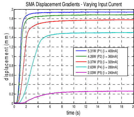
Figure 6: SMA Displacement Gradients
