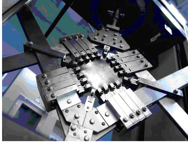
Figure 11. A stretch frame used for equi-biaxial loading of rubber specimens.
