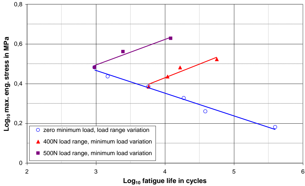
Figure 5. \text{Log}_{10} of the maximum engineering (nominal) stress versus \text{log}_{10} of number of cycles to failure for filled EPDM for various load ranges and minimum loads.
