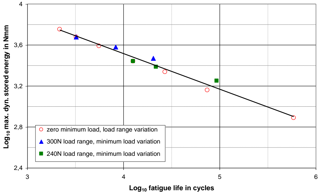
Figure 3. \text{Log}_{10} of maximum dynamic energy versus \text{log}_{10} of number of cycles to failure for filled SBR for various load ranges and minimum loads.
