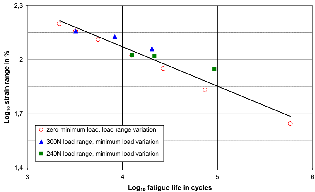
Figure 4. \text{Log}_{10} of the strain range against \text{log}_{10} of number of cycles to failure for filled SBR for various load ranges and minimum loads.
