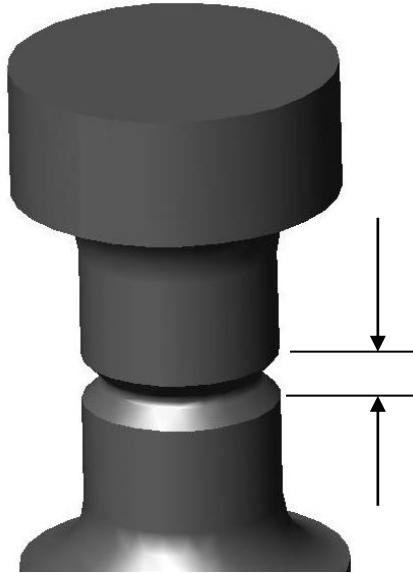
Figure 8. A diagrammatic representation of a dumbbell specimen. The volume of the critical region is indicated as that confined to the notch as shown.
