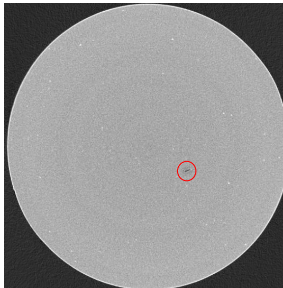
Figure 9. X-ray of a 15 mm diameter dumbbell sample showing particles of various sizes. (A flaw of approximately 500\text{ }\mu\text{m} in length can be seen close to the sample centre. The image is reproduced from an analysis performed by S. Robin).
