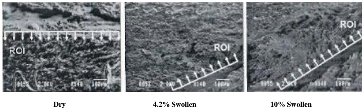
Figure 26. SEM Imaging of specimen fracture surfaces, \sigma_{\text{eng}} = 1 \text{ MPa} (ROI = Region of interest).
