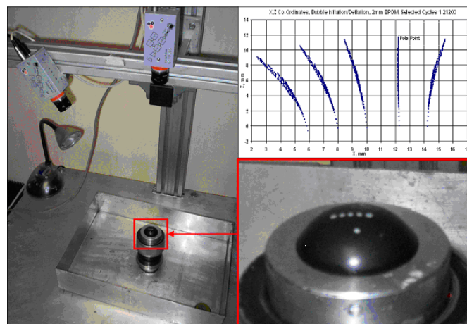
Figure 13. The final configuration of the equi-biaxial bubble inflation test system.
