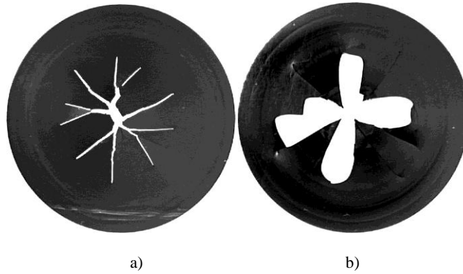
Figure 12. Failure of statically inflated HNBR 50 mm samples, a) hydraulically inflated and b) pneumatically inflated
