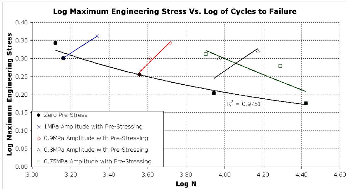
Figure 18. S-N curve for EPDM samples with and without pre-stressing, using \sigma_{\text{eng}} = P R \lambda_1/2 t_0 control.
