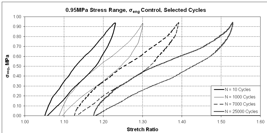
Figure 17. Hysteresis curves for selected cycles in a fatigue test on an EPDM sample.
